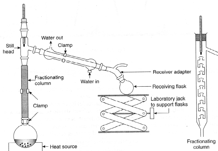
FRACTIONAL DISTILLATION
