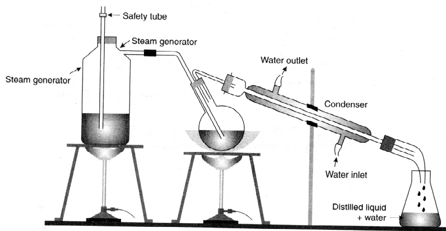
STEAM DISTILLATION
